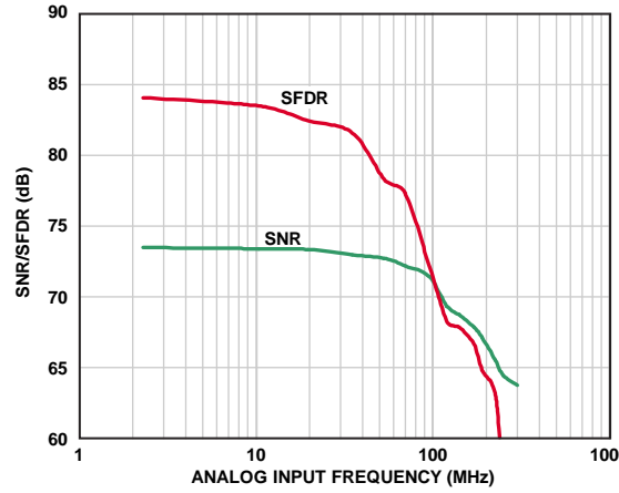
Figure 25. SNR/SFDR vs. f_{IN} , f_{SAMPLE} = 50 \text{ MSPS}
