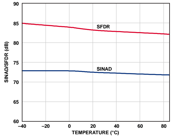
Figure 26. SINAD/SFDR vs. Temperature, f_{IN} = 19.7 \text{ MHz} , f_{SAMPLE} = 50 \text{ MSPS}
